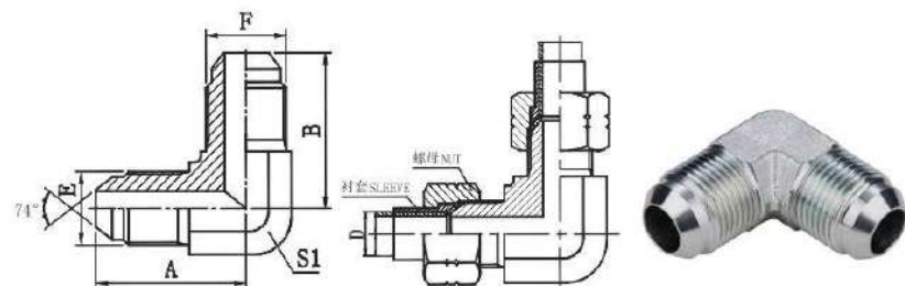
1J9 90° 弯美制JIC外螺纹74° 外锥 90° ELBOW JIC MALE 74° CONE
