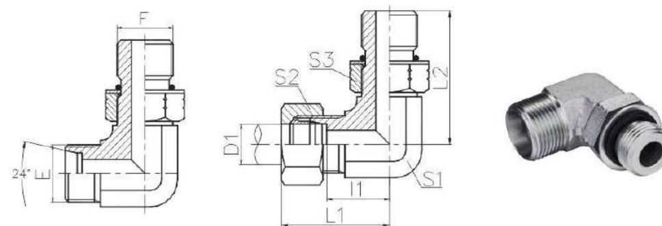
90° 弯美制螺纹可调向O形圈密封柱端ISO 11926 90° ELBOW UN、UNF THREAD ADJUSTABLE STUD ENDS WITH O-RING SEALING ISO 11926
