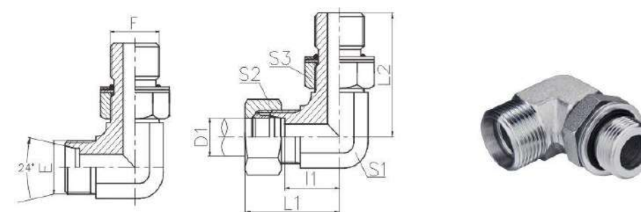
90° 弯英管螺纹可调向O形圈密封柱端 90° ELBOW BSPP THREAD ADJUSTABLE STUD ENDS WITH O-RING SEALING
