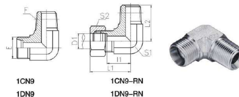
90° 弯布锥管外螺纹 90° ELBOW NPT MALE
