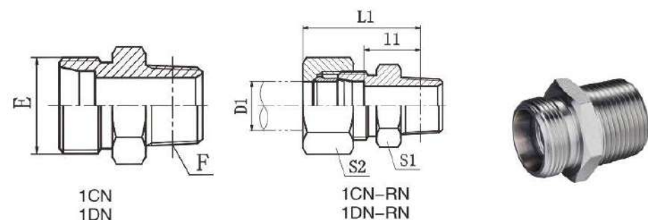
布锥管外螺纹 NPT MALE
