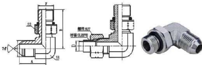
90° 弯美制JIC外螺纹74° 外锥/ SAE外螺纹带O形圈轻系列ISO 11926-3 90° ELBOW JIC MALE 74° CONE /SAE O-RING BOSS L-SERIES ISO 11926-3
