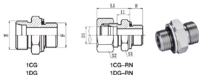
英管螺纹O形圈密封柱端 BSPP THREAD STUD ENDS WITH O-RING SEALING
