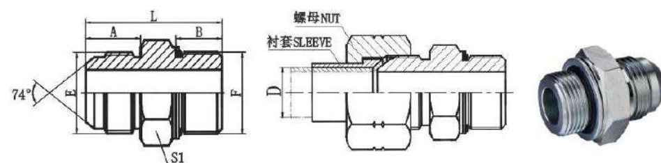
1JG 美制JIC外螺纹74° 外锥/ 英管外螺纹O形圈 JIC MALE 74° CONE / BSPP MALE O-RING
