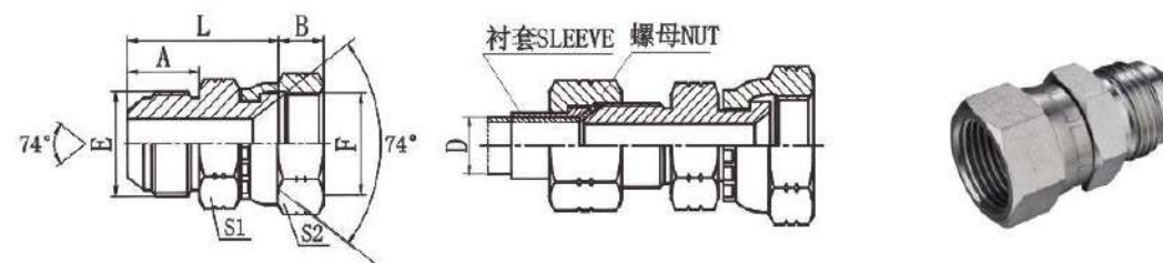
2J 美制JIC外螺纹74° 外锥/JIC内螺纹74° 内锥 JIC MALE 74° CONE / JIC FEMALE 74° SEAT
