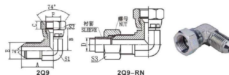
公制外螺纹74° 外锥 公制内螺纹74° 内锥 METRIC MALE 74° CONE METRIC FEMALE 74° SEAT
