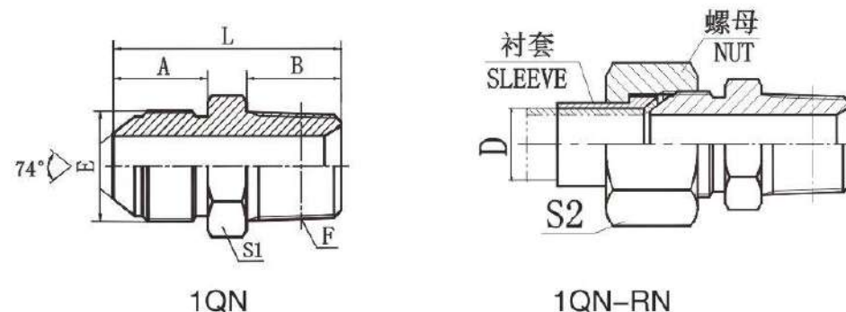
公制外螺纹74° 外锥/布锥管外螺纹 METRIC MALE 74° CONE/NPT MALE
