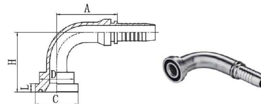
87391 90° SAE 法兰3000 PSI 90° SAE FLANGE 3000 PSI ISO12151-3-SAE J516
