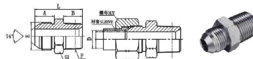
JIC外螺纹74° 外锥/ 布锥管外螺纹 JIC MALE 74° CONE / NPT MALE
