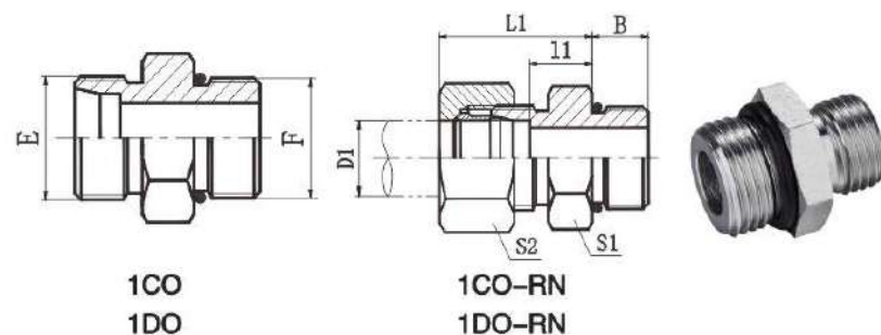
美制螺纹O形圈密封柱端ISO 11926 UN、UNF THREAD STUD ENDS WITH O-RING SEALING ISO 11926
