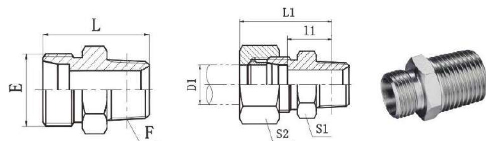
英锥管外螺纹 BSPT MALE
